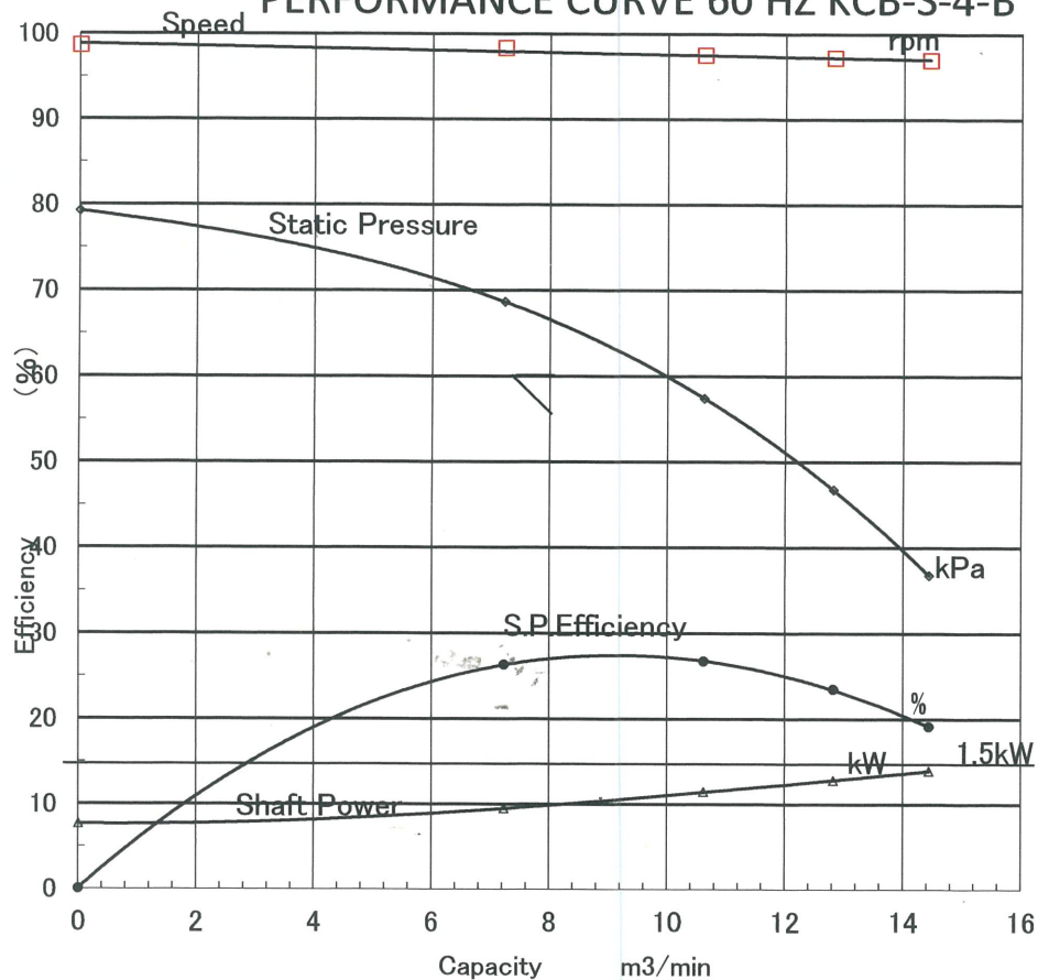
PERFORMANCE CURVE 60 HZ KCB-S-4-B
