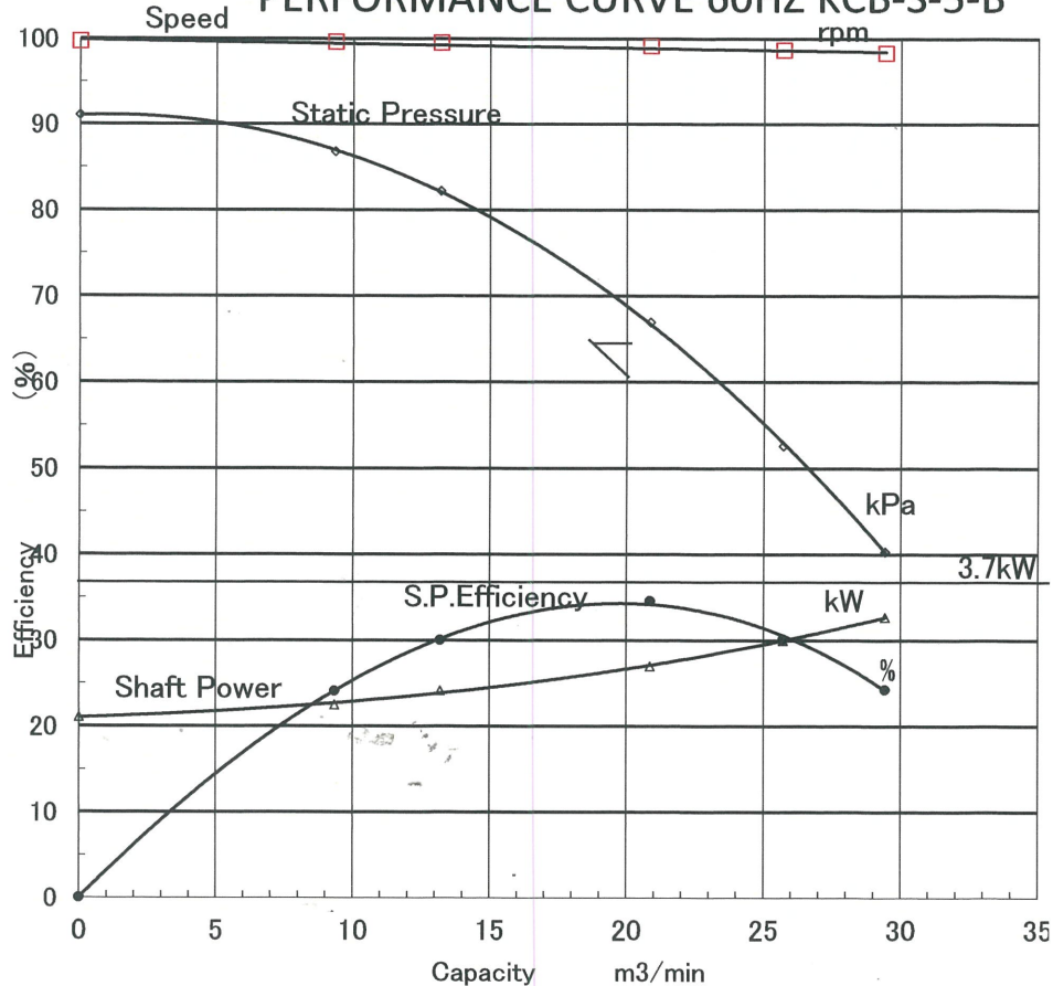
PERFORMANCE CURVE 60HZ KCB-S-5-B
