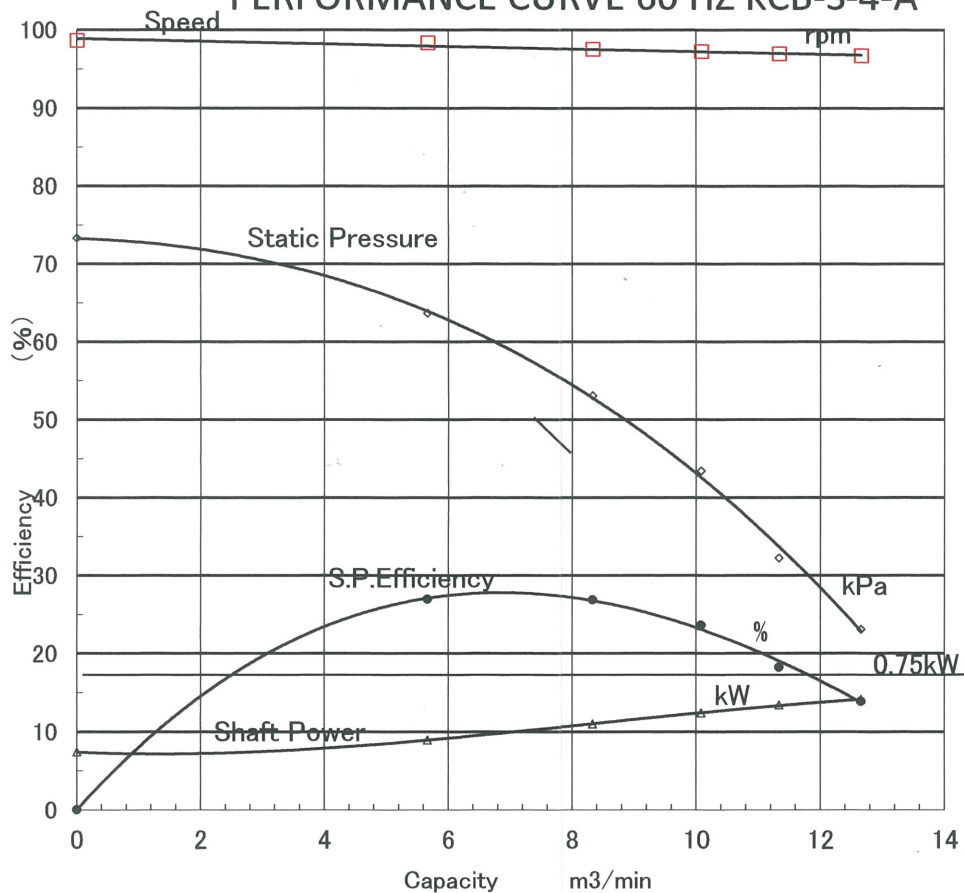
PERFORMANCE CURVE 60 HZ KCB-S-4-A
