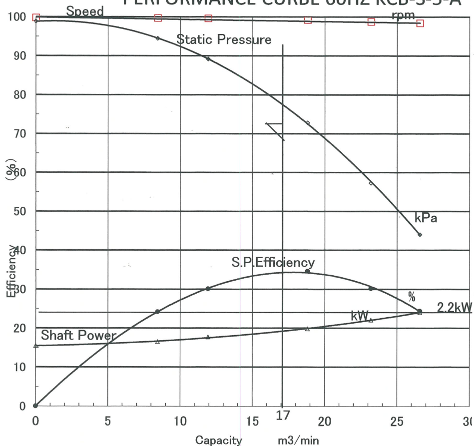
PERFORMANCE CURBE 60HZ KCB-S-5-A
